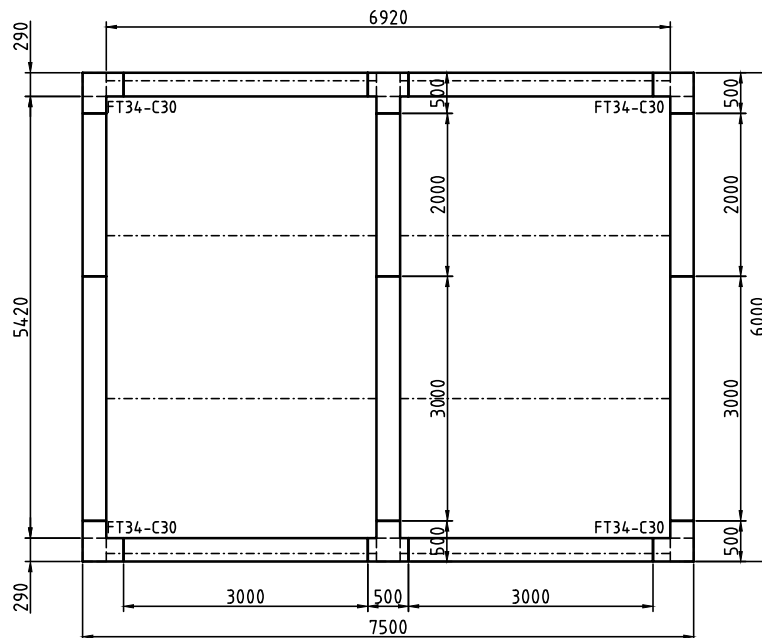
GROUND PLAN
